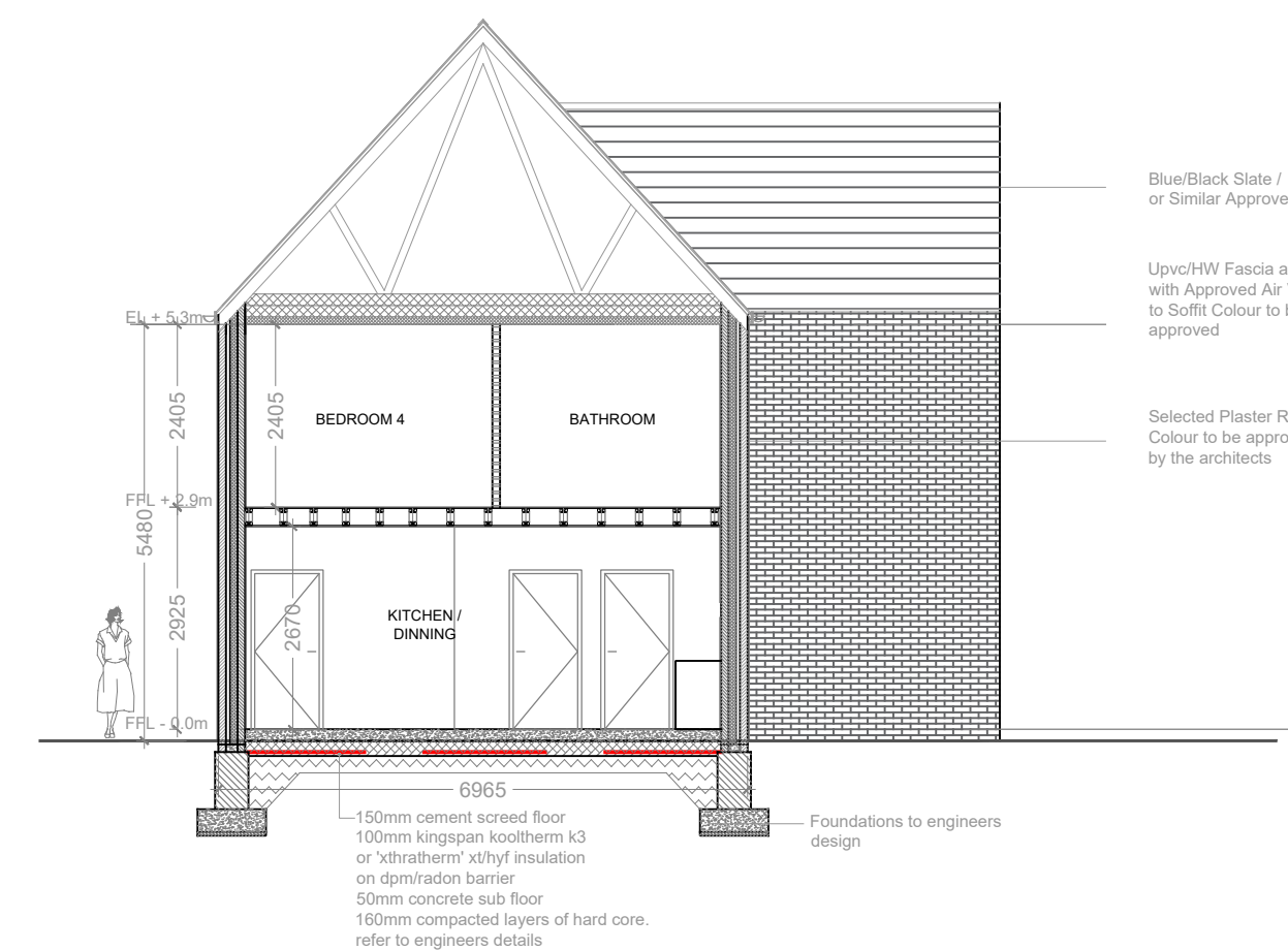
09 SECTION-B BLOCK-2 1:100
