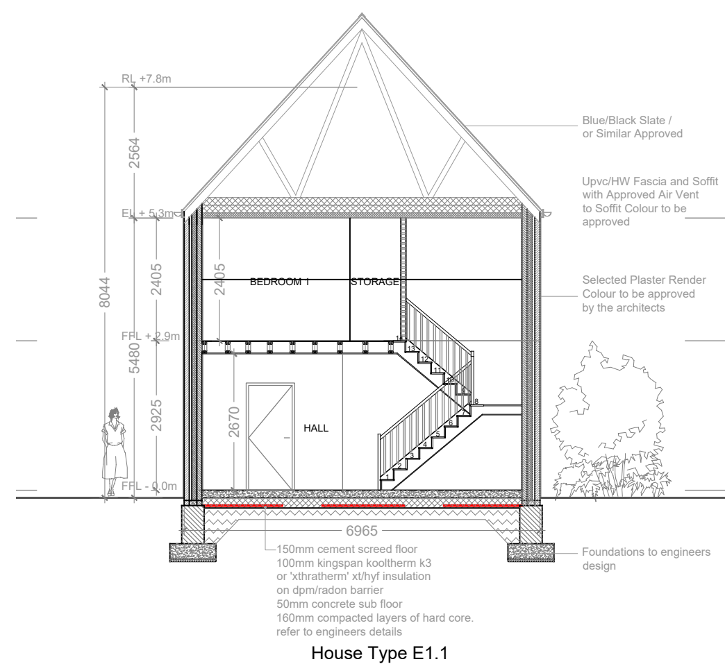
08 SECTION-A BLOCK-2 1:100
